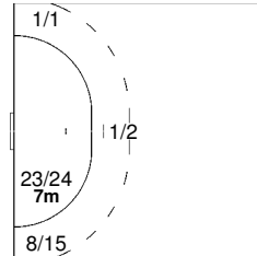
9 CHRISTIANSEN Lars
