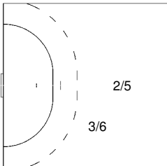
18 RUDOVIC Novica
