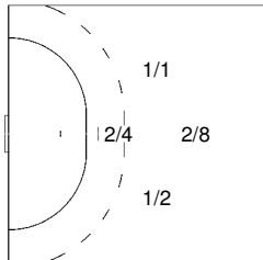
23 ZORMAN Uros
