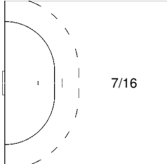
2 SOLBERG Glenn
