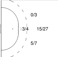
2 BOQUIST Martin
