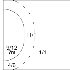
4 KOKSHAROV Eduard
