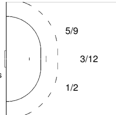
10 ROGANOVIC Zoran
