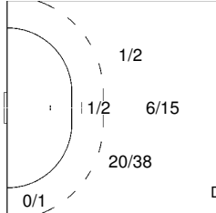
3 HAGEN Frode
