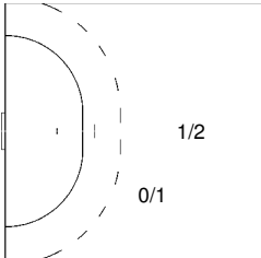
5 ASTROUSKI Vasili
