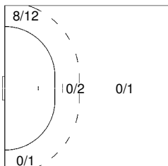
20 SKJÆRVOLD Rune
