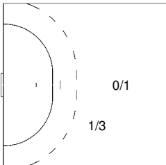
24 STRANOVSKY Martin
