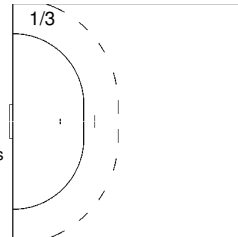
17 GAJIC Dragan
