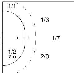
30 GUILBERT Fabrice
