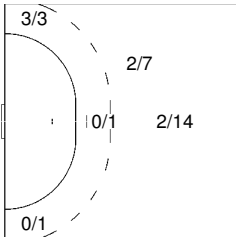
14 ZEITZ Christian
