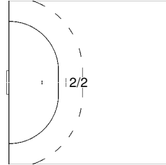
4 BABICHEV Maxim
