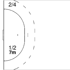
4 DOBRKOVIC Marko
