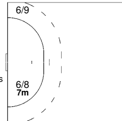
27 CUPIC Ivan
